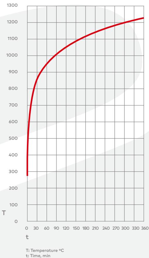
*Figure-1: Standard Temperature / Time Curve According to EN 1363-1 (ISO 834)
